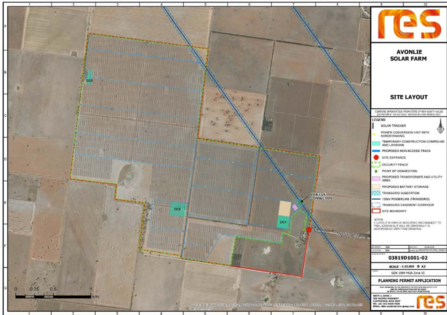
Figure 3. Proposal area layout
