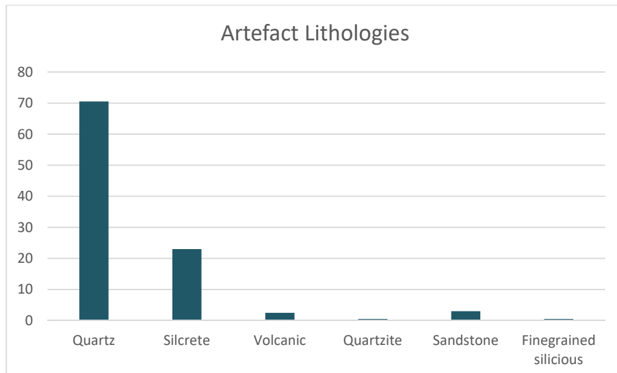
Figure 8 Artefact Lithology
