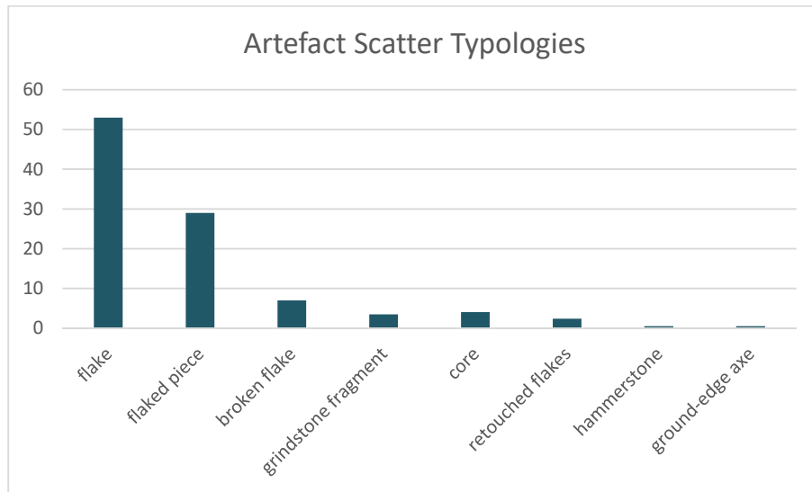
Figure 7 Artefact Typology
